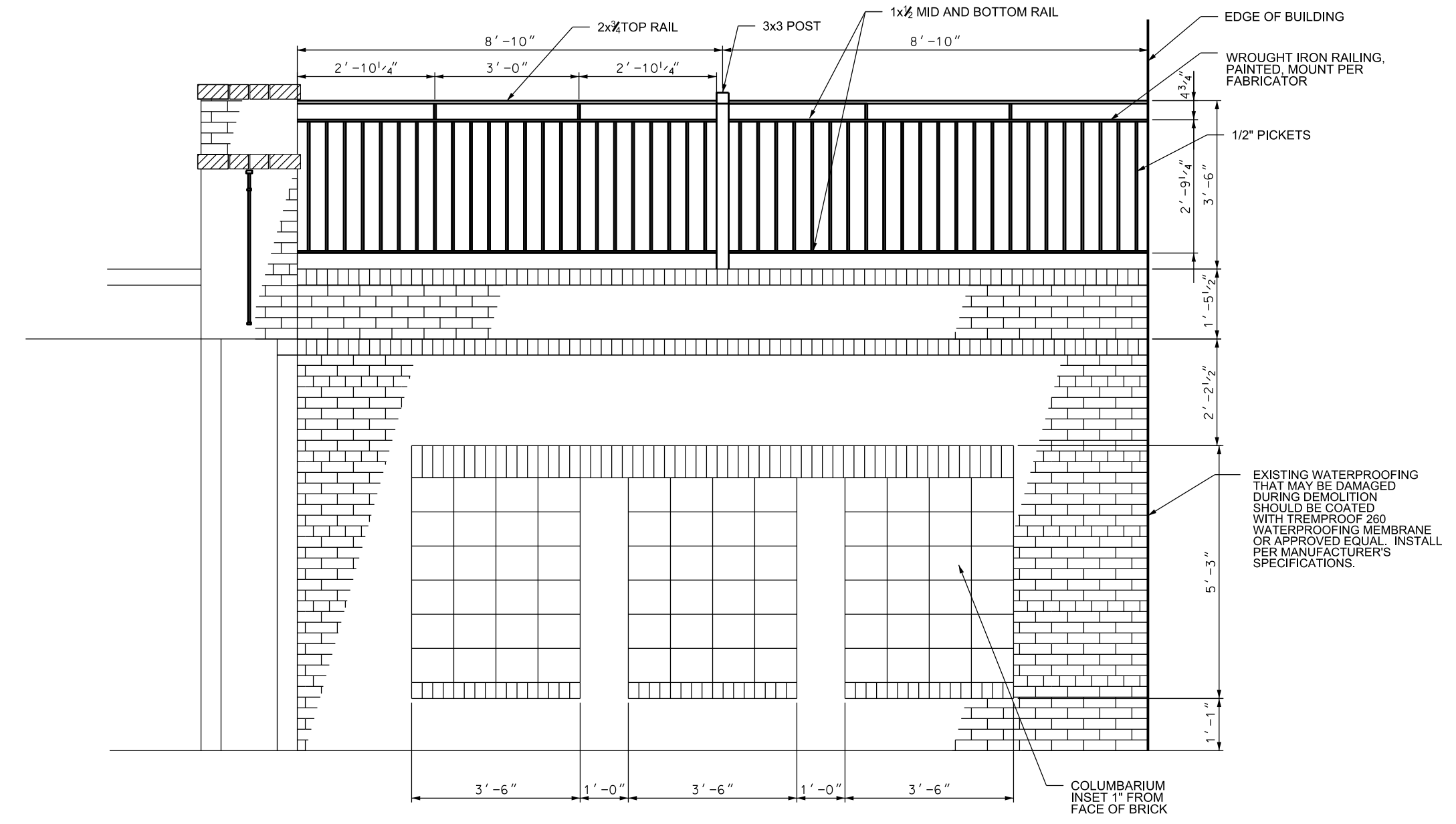
1 PARTIAL ELEVATION L2 SCALE: 3/4" = 1'-0"
